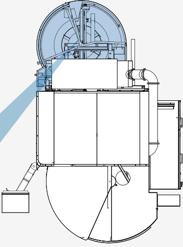
Mikron MILL X 600 U: disc-type magazine
